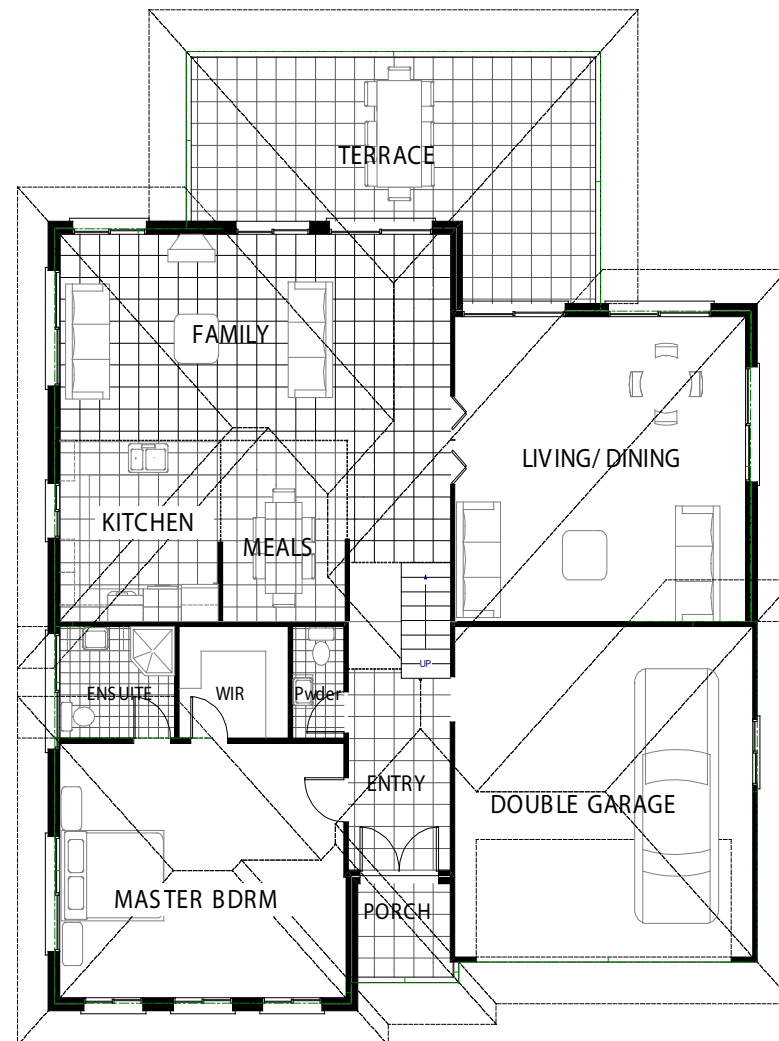
LOWER FLOOR
